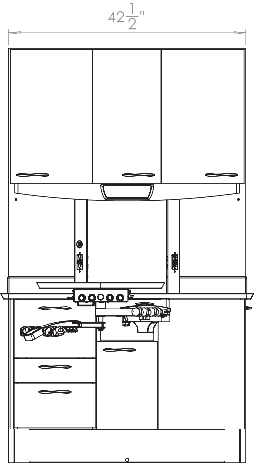
42" Wall Mounted 12 O'Clock Dimensions
